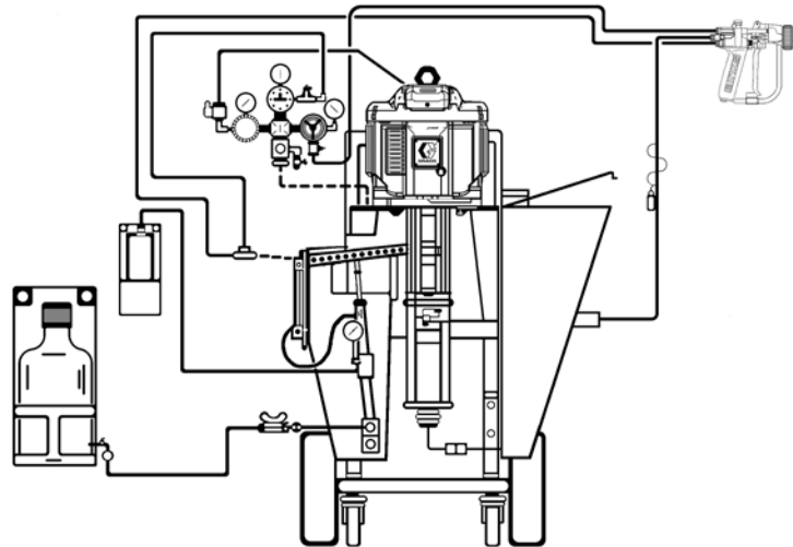
SPRAY-QUIP 398-275 CATALYST INJECTION SYSTEM
